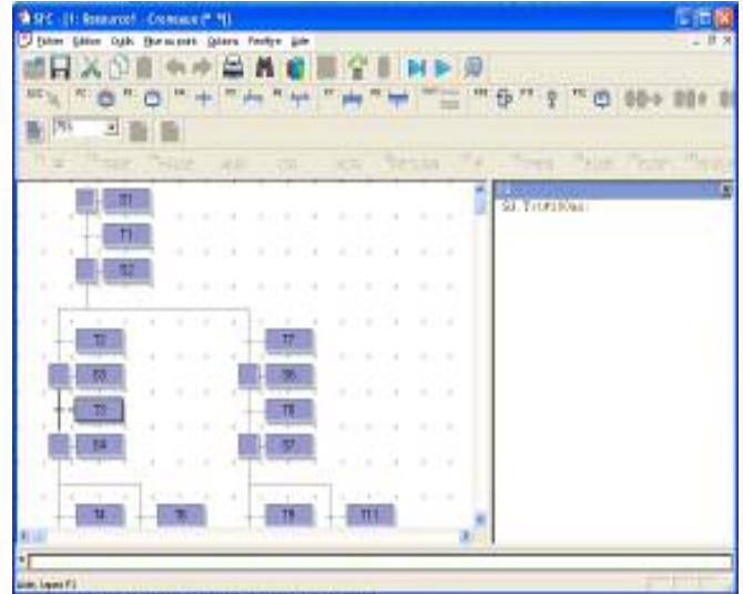
SFC language
