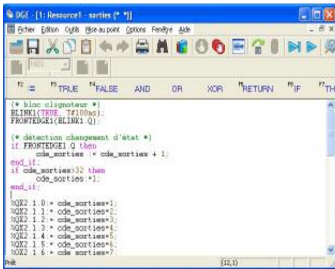
Structured Text language Syntactical coloration
